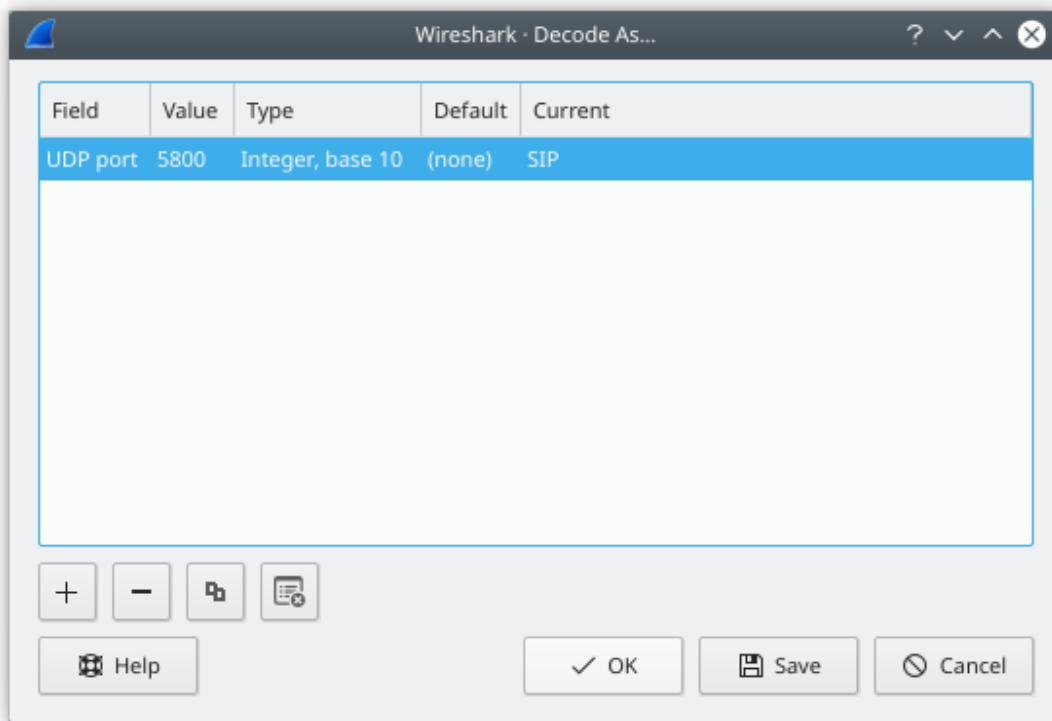
Figure 124. The “Decode As” dialog box
